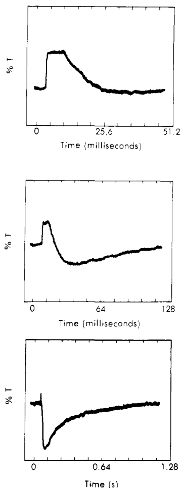
Figure 1. Typical traces of percent transmittance at 500 nm vs. time for the \text{Fe}^{\text{II}}\text{TMP-HNO}_2 reaction using three different time spans. Note how the shortest time span shows only the first phase, while the longest enables us to focus on the second (recovery) phase.
