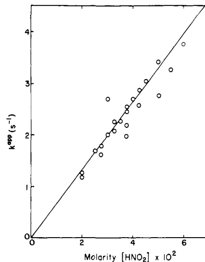
Figure 4. [\text{HNO}_2] dependence of k^{\text{app}} for phase 2. [\text{Fe}^{\text{II}}\text{TMP}]_0 = 1.0 \times 10^{-4} M, [\text{HCl}]_0 = [\text{NaNO}_2]_0 .
