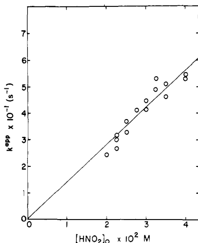
Figure 3. [\text{HNO}_2] dependence of k^{\text{app}} for phase 1. [\text{Fe}^{\text{II}}\text{TMP}]_0 = 1.0 \times 10^{-4} M, [\text{HCl}]_0 = [\text{NaNO}_2]_0 = 0.02 M.
